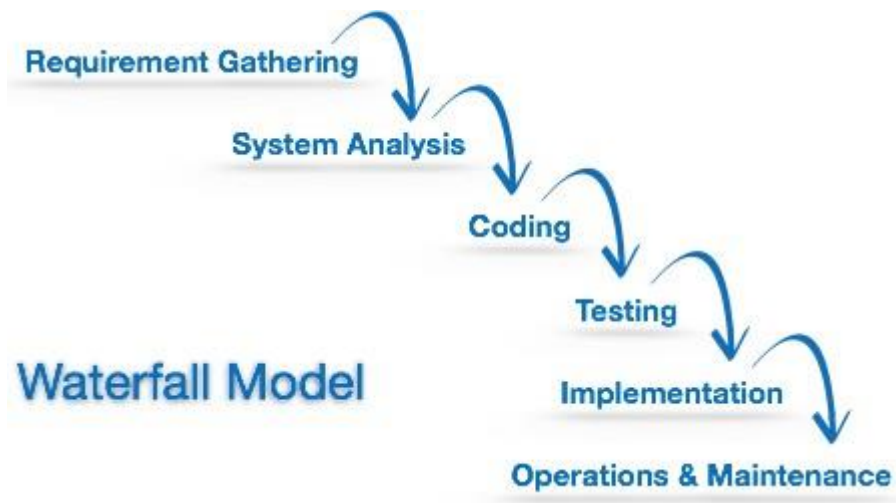
Fig 2: Waterfall Model
